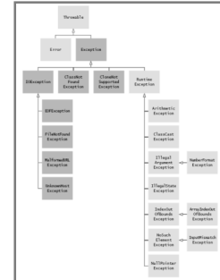
Figure 1: The Hierarchy of Exception Classes
